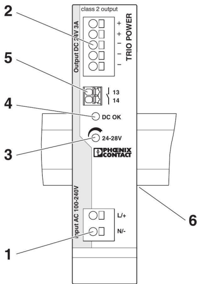
Figure 2 Function elements
