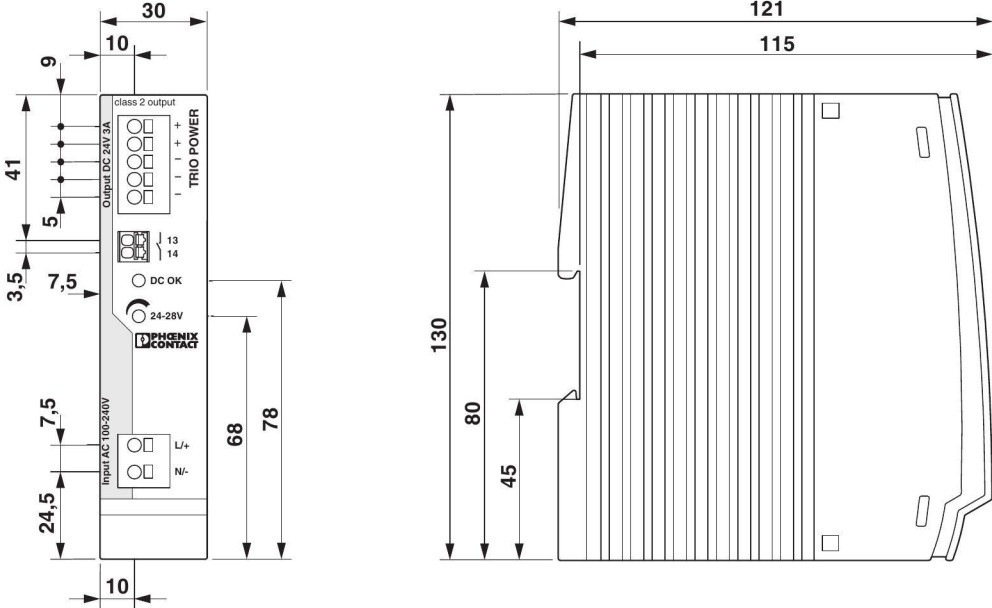
Figure 5 Device dimensions
